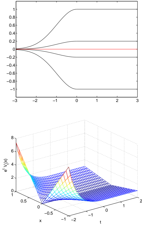
Figure 6: Phase portrait (left) and (t, x) \mapsto e^t V_t(x) (right) for Example 26
