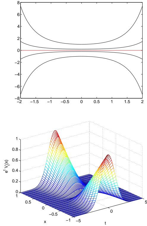
Figure 3: Phase portrait (left) and (t, x) \mapsto e^t V_t(x) (right) for Example 23
