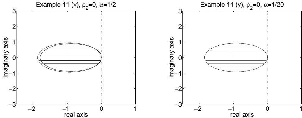
Figure 3: Two stability regions as described in Example 11 (v) with rational \alpha .
