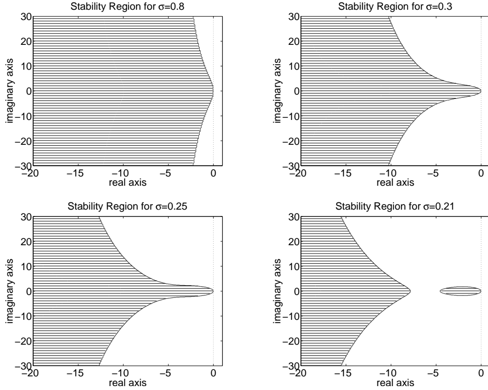
Figure 1: Stability regions as described in Example 11 (iv) for different values of \sigma
