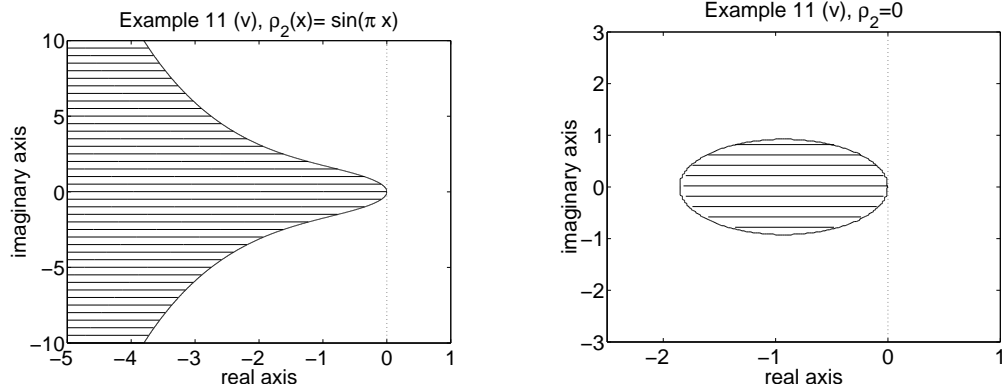
Figure 2: Two stability regions as described in Example 11 (v) with our without continuous intervals
