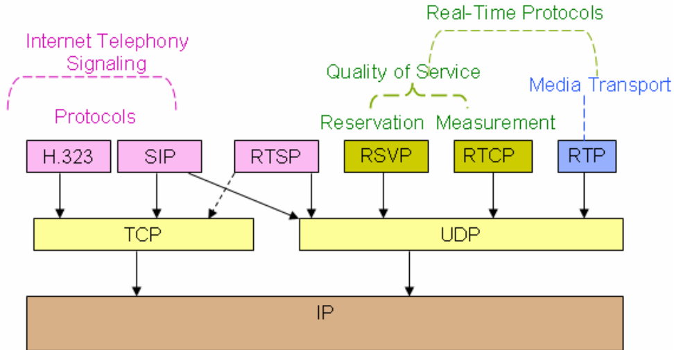
Figure 2. Protocol Suite
